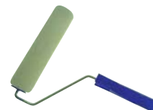
PM914 9" Complete set: Roller refill: Polyester fabric, Pile Height:14mm, PP Core, Dia:38mm. Roller Frame:4 Cages wire, main rod chrome tinplated with dia 6mm, blue plastic handle
